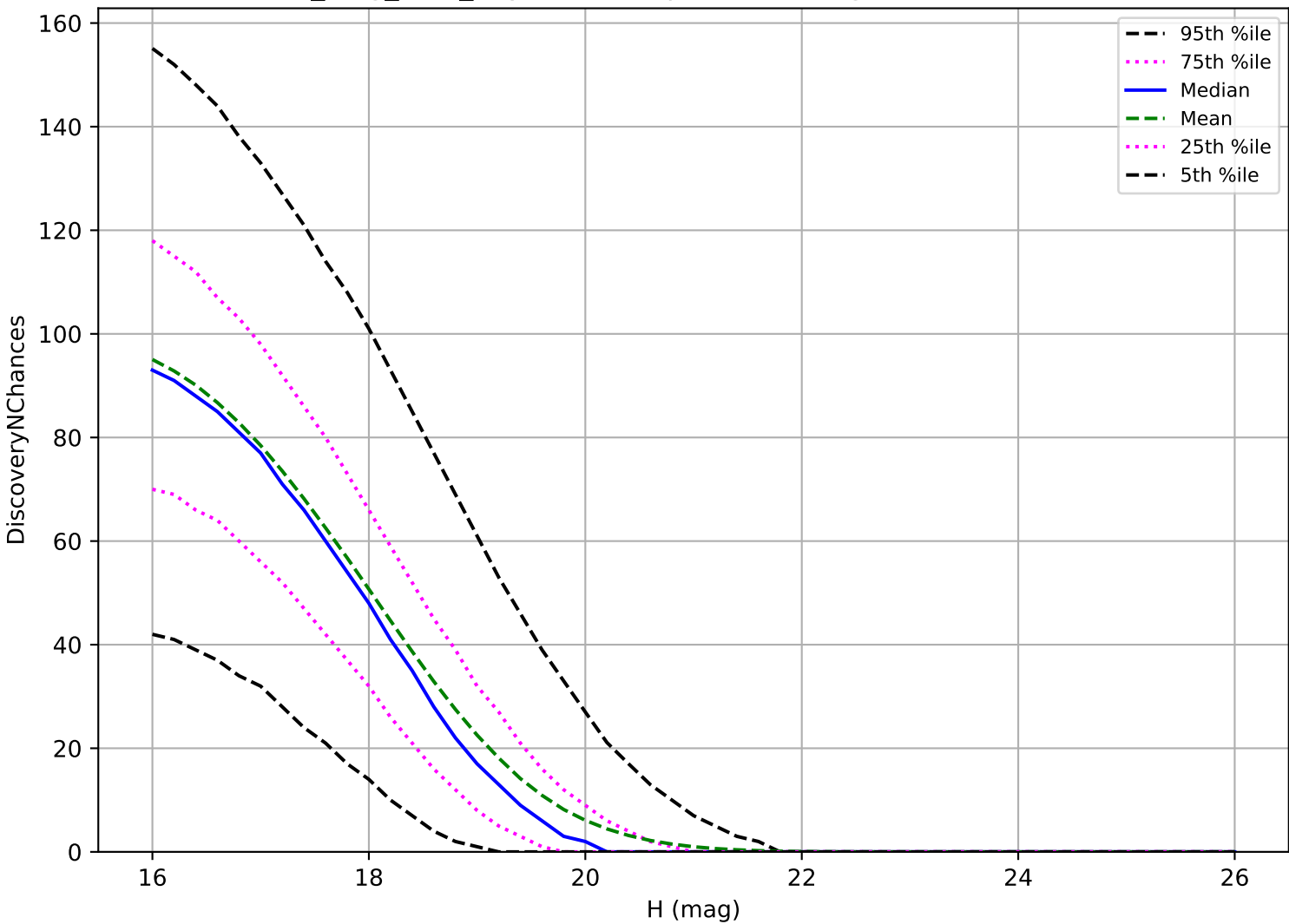
no_long_v3.4_10yrs: MBA 3 pairs in 15 nights detection loss
