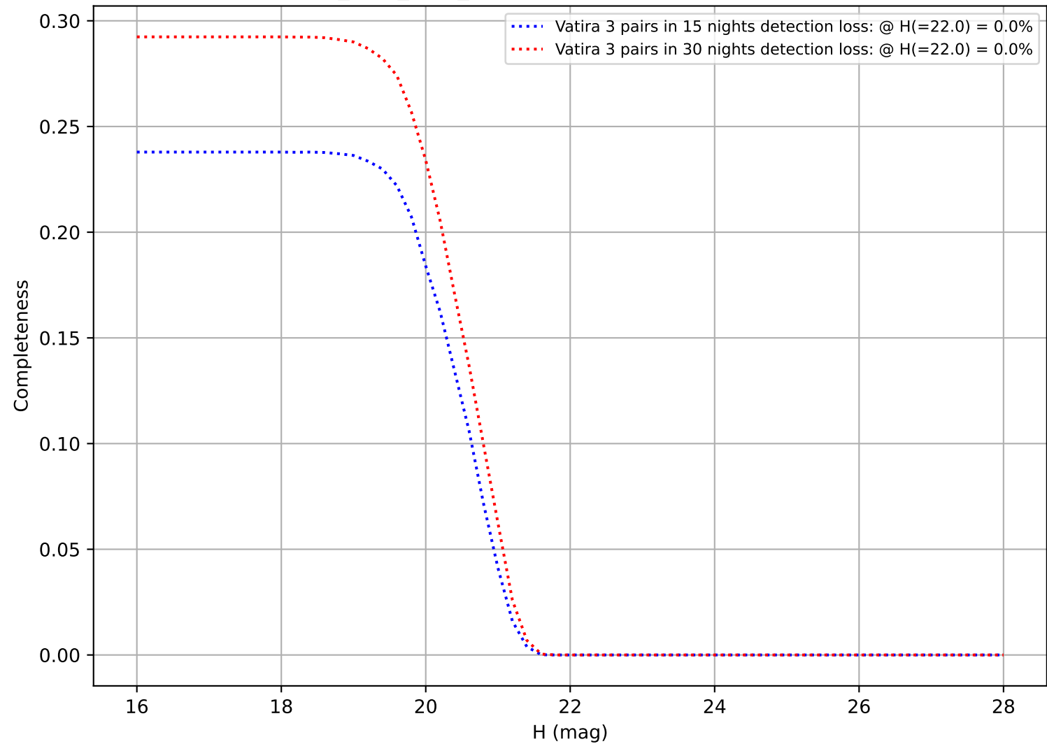
no_long_v3.4_10yrs: DifferentialCompleteness
