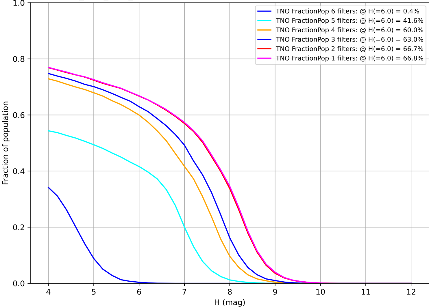
no_long_v3.4_10yrs: Fraction of population with colors in X filters TNO
