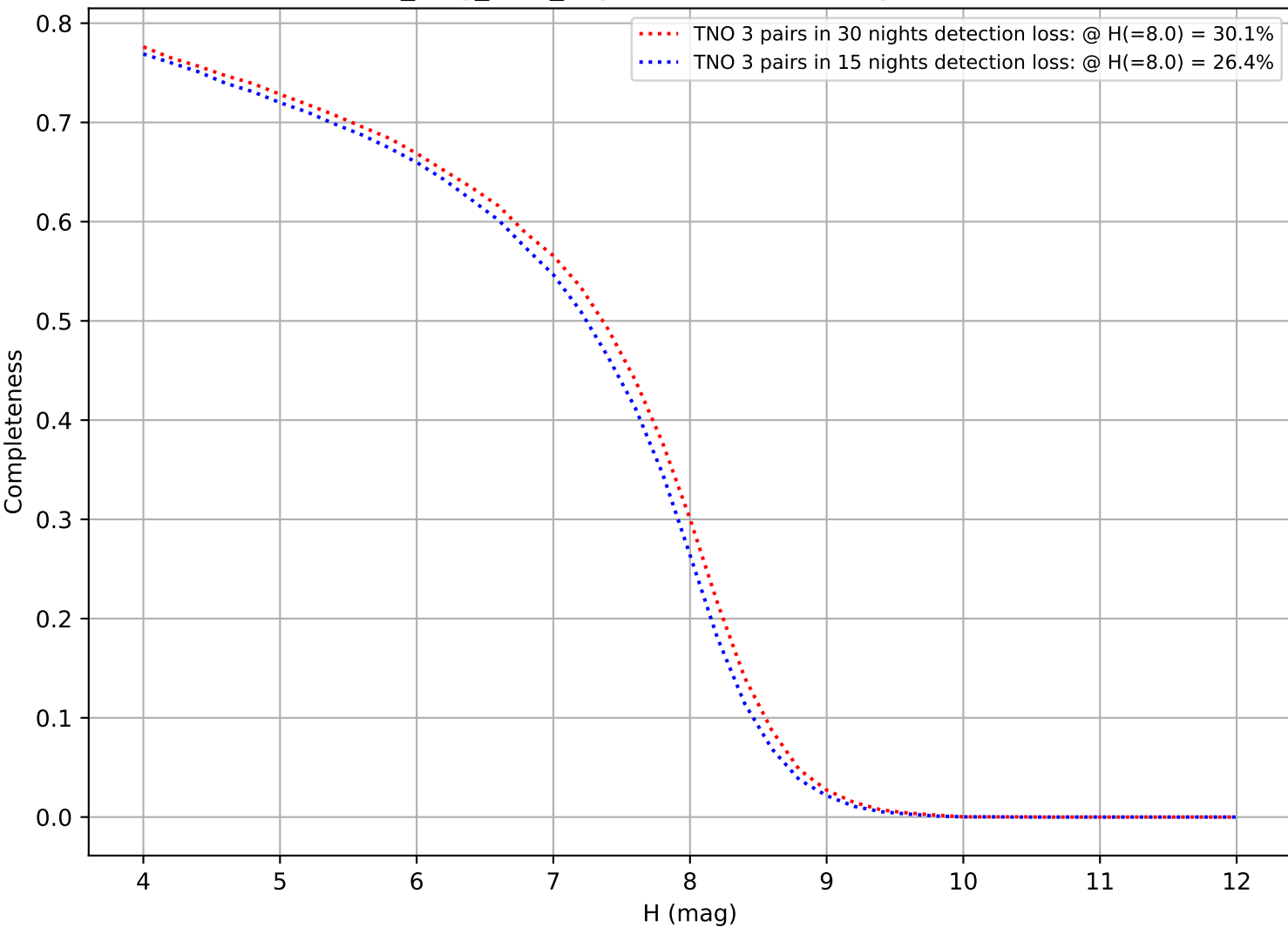
no_long_v3.4_10yrs: DifferentialCompleteness
