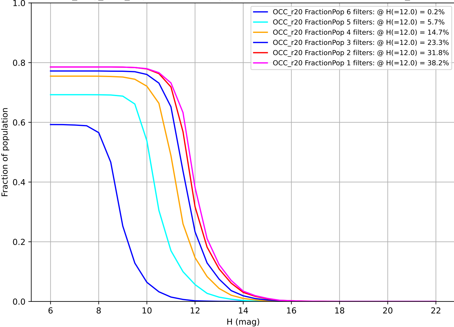
no_long_v3.4_10yrs: Fraction of population with colors in X filters OCC_r20
