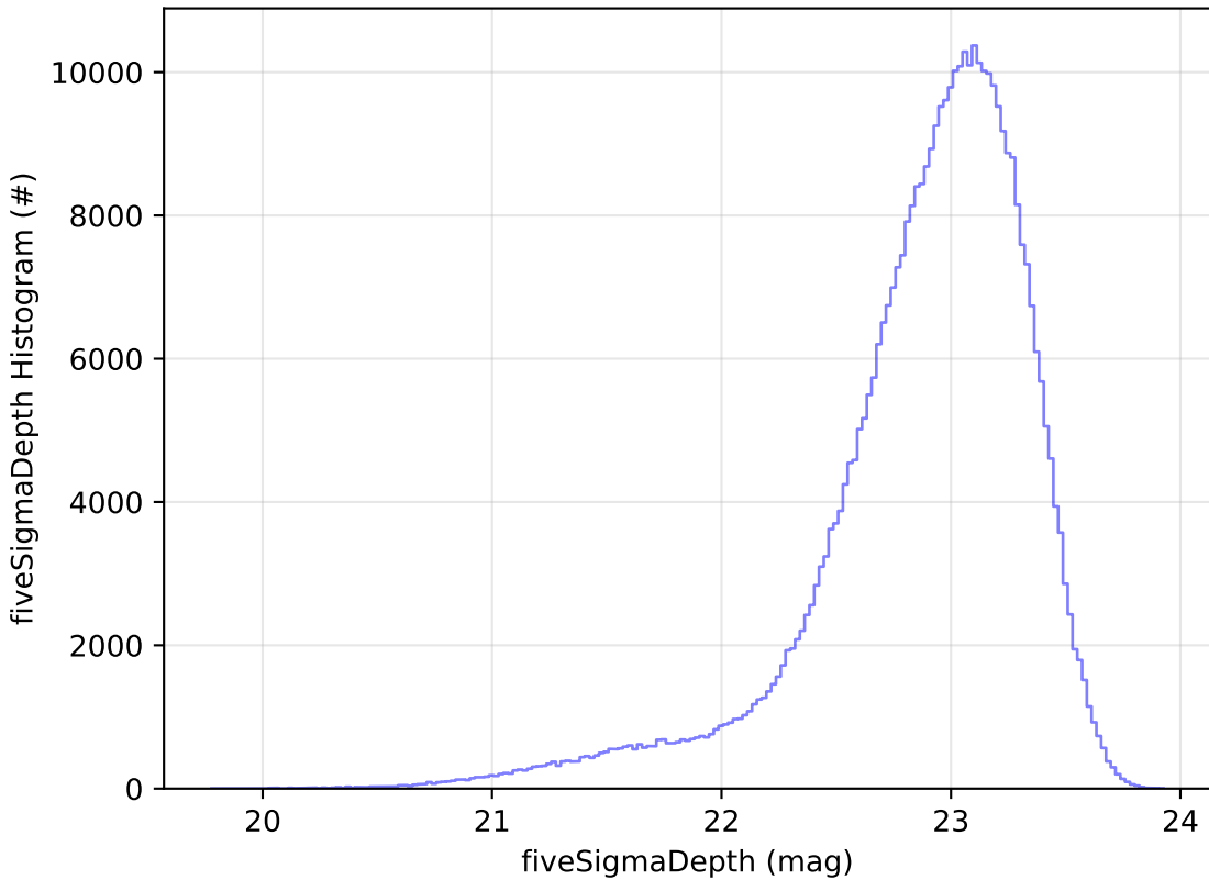
no_long_v3.4_10yrs z: fiveSigmaDepth Histogram
