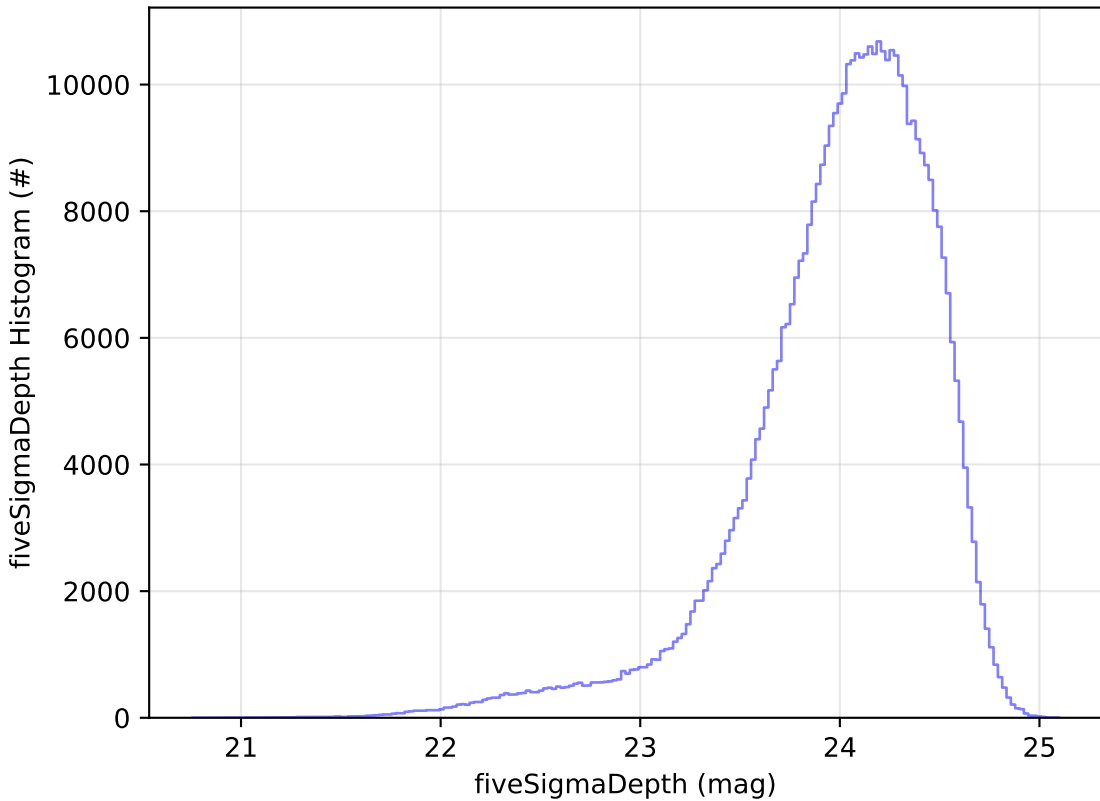
no_long_v3.4_10yrs r: fiveSigmaDepth Histogram
