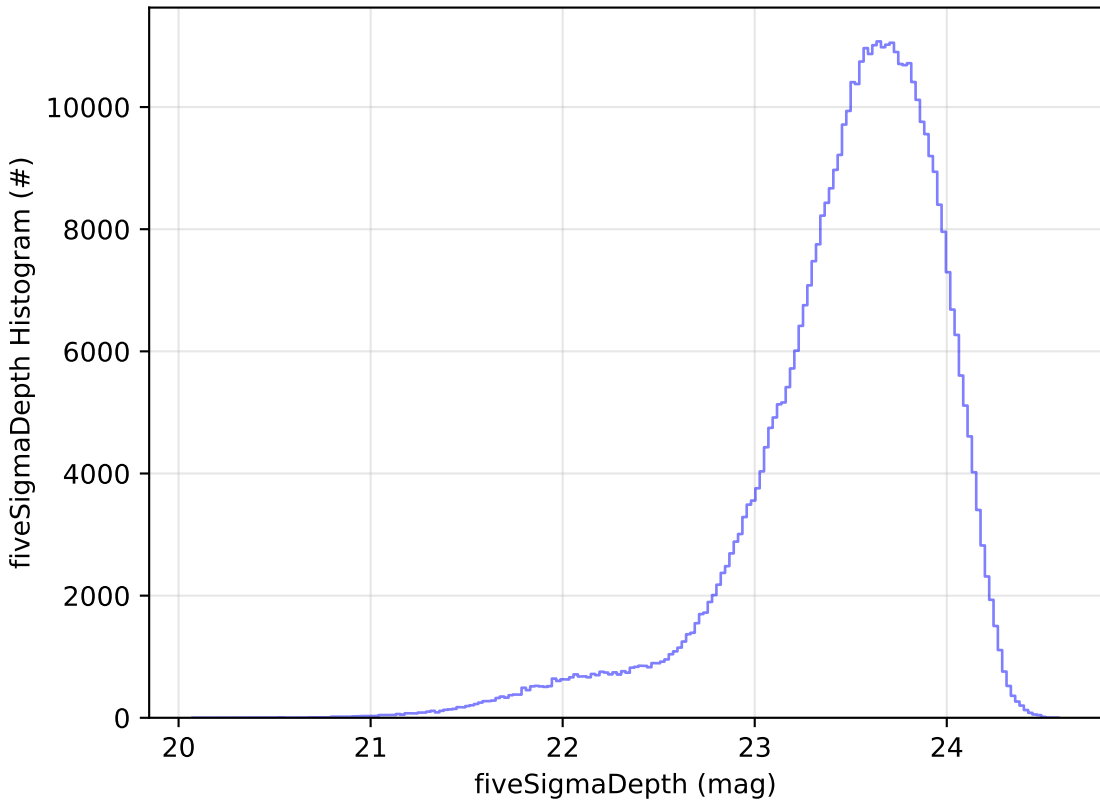
no_long_v3.4_10yrs i: fiveSigmaDepth Histogram
