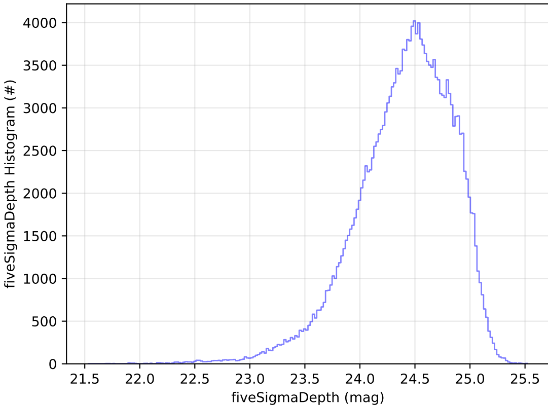
no_long_v3.4_10yrs g: fiveSigmaDepth Histogram
