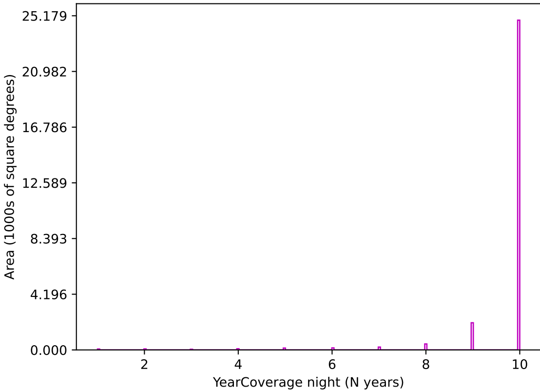
no_long_v3.4_10yrs z band: YearCoverage night
