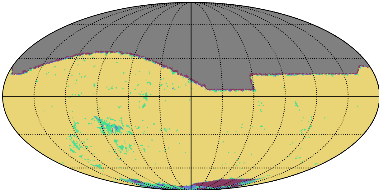
no_long_v3.4_10yrs r band: YearCoverage night
