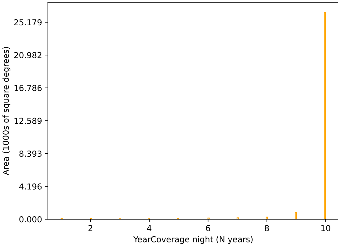
no_long_v3.4_10yrs r band: YearCoverage night
