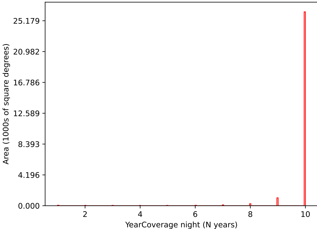
no_long_v3.4_10yrs i band: YearCoverage night
