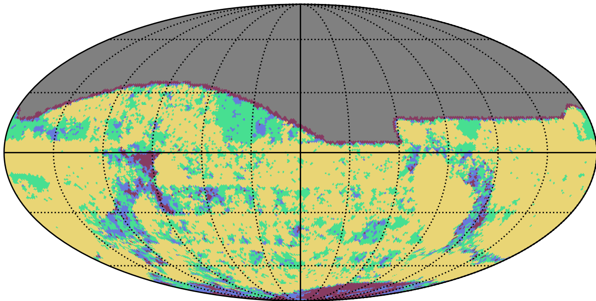
no_long_v3.4_10yrs g band: YearCoverage night
