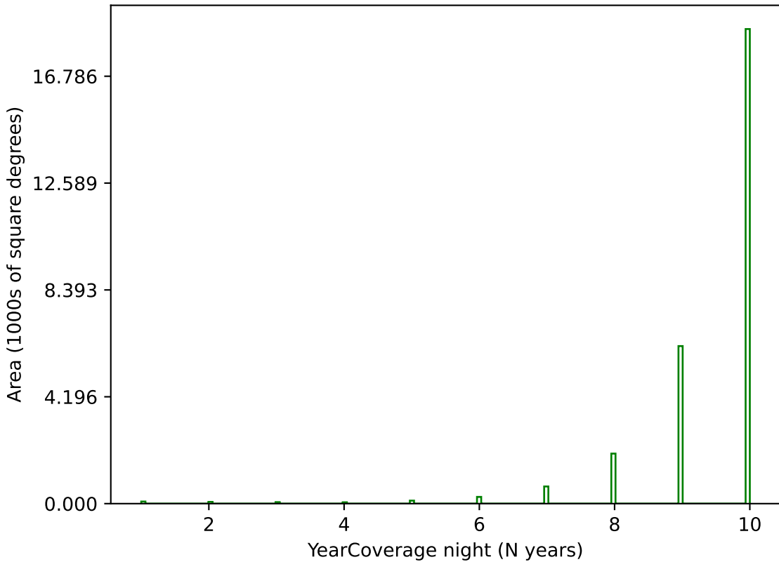
no_long_v3.4_10yrs g band: YearCoverage night
