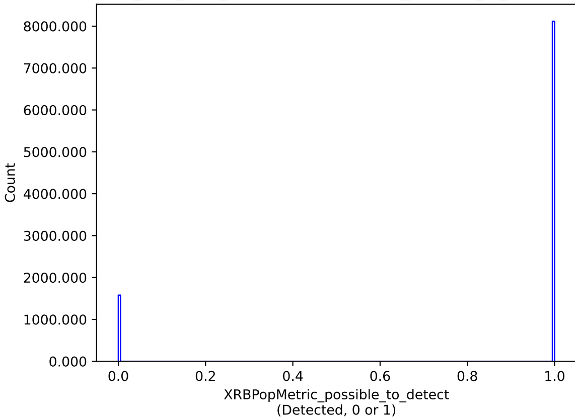
no_long_v3.4_10yrs : XRBPoMetric_possible_to_detect
