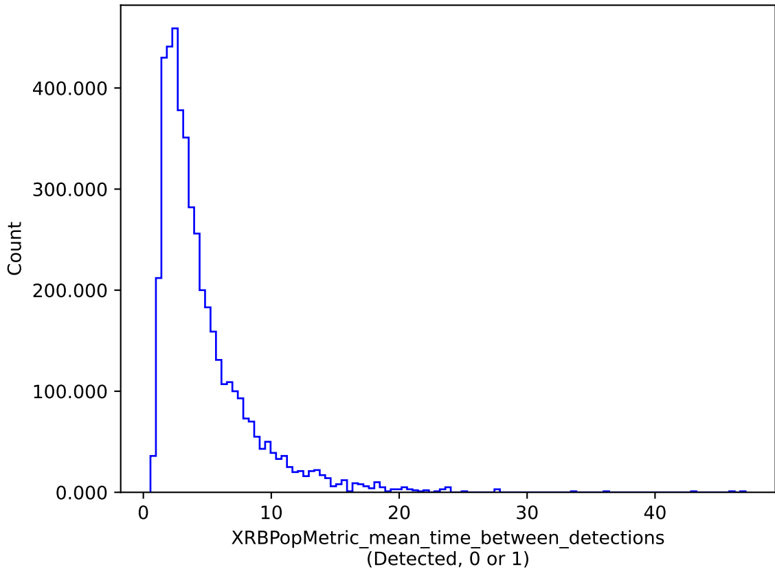
no_long_v3.4_10yrs : XRBPoMetric_mean_time_between_detections
