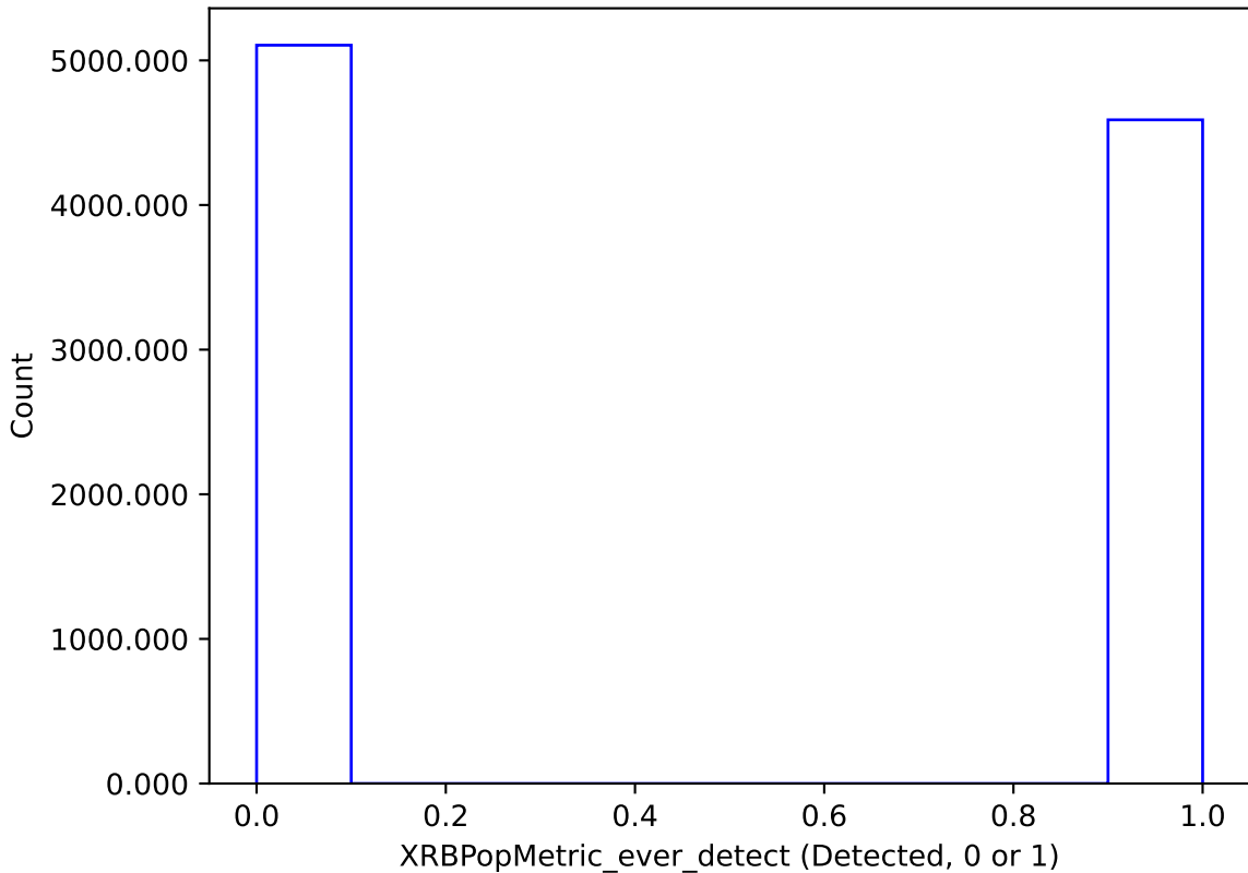
no_long_v3.4_10yrs : XRBPoMetric_ever_detect
