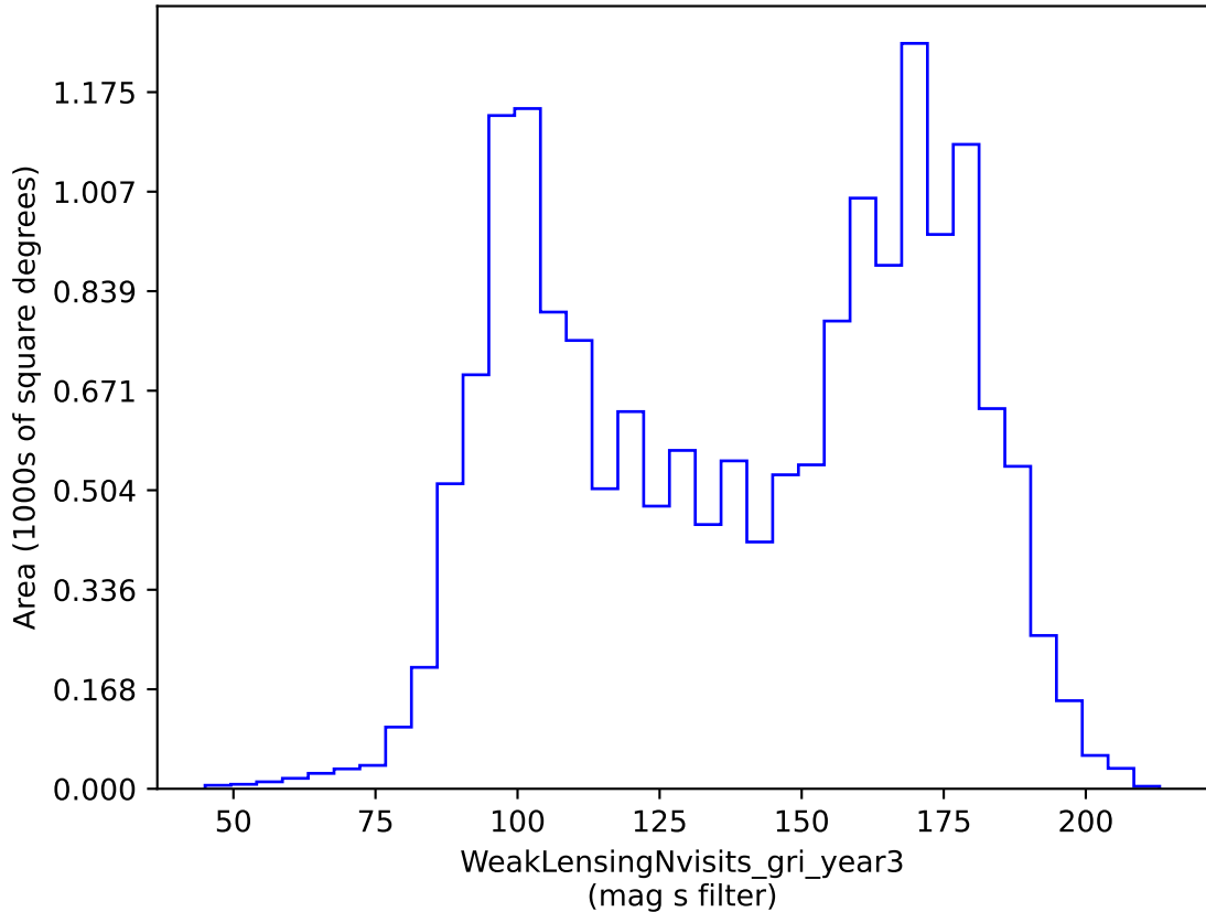
no_long_v3.4_10yrs gri band non-DD: WeakLensingNvisits_gri_year3
