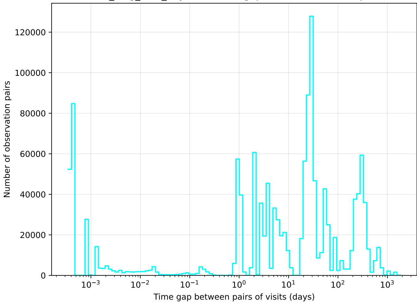
no_long_v3.4_10yrs u band: Tgaps observationStartMJD
