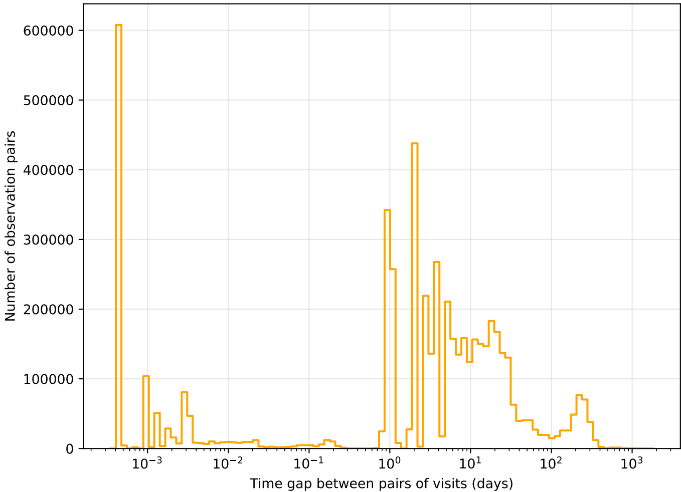
no_long_v3.4_10yrs r band: Tgaps observationStartMJD
