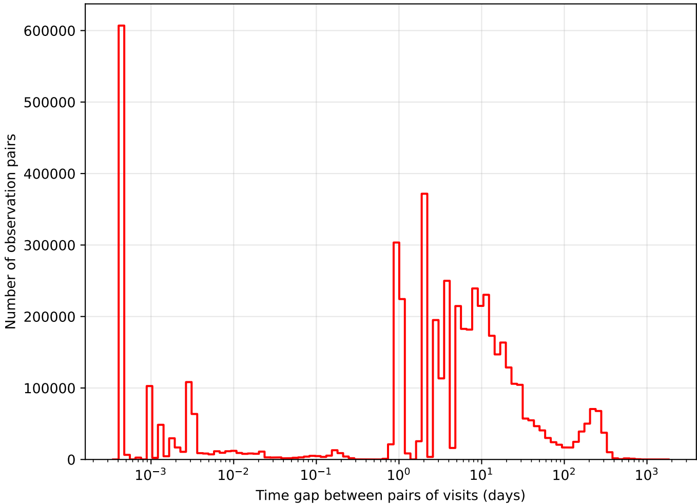
no_long_v3.4_10yrs i band: Tgaps observationStartMJD
