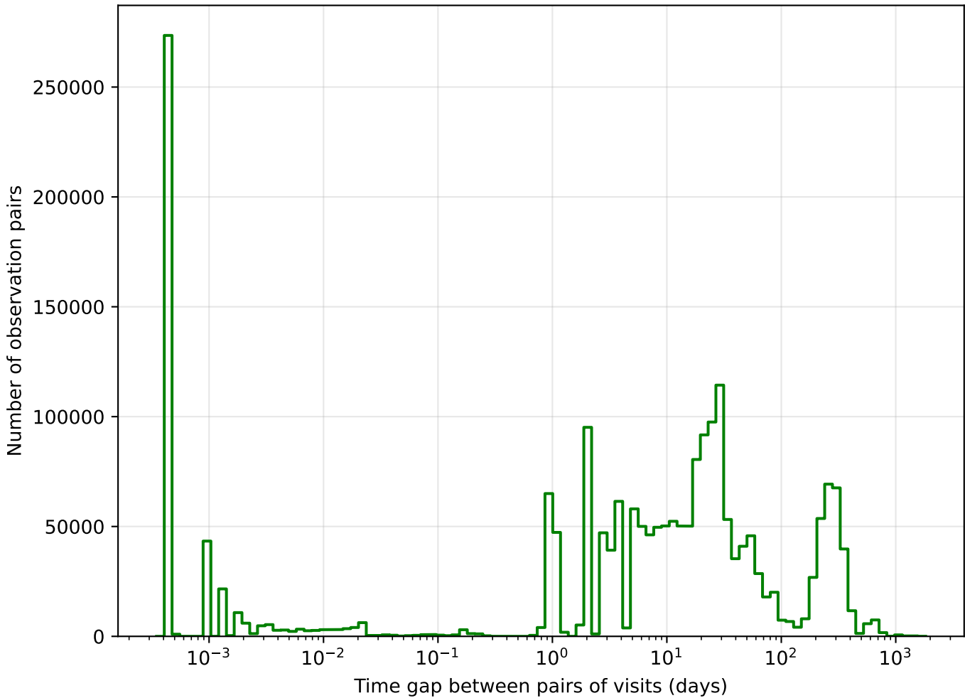
no_long_v3.4_10yrs g band: Tgaps observationStartMJD
