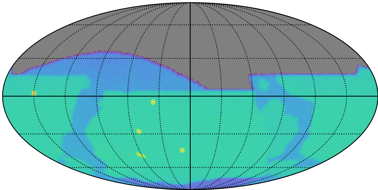
no_long_v3.4_10yrs z: SurfaceBrightLimit
