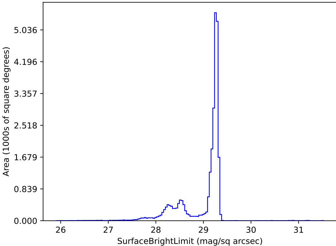
no_long_v3.4_10yrs z: SurfaceBrightLimit
