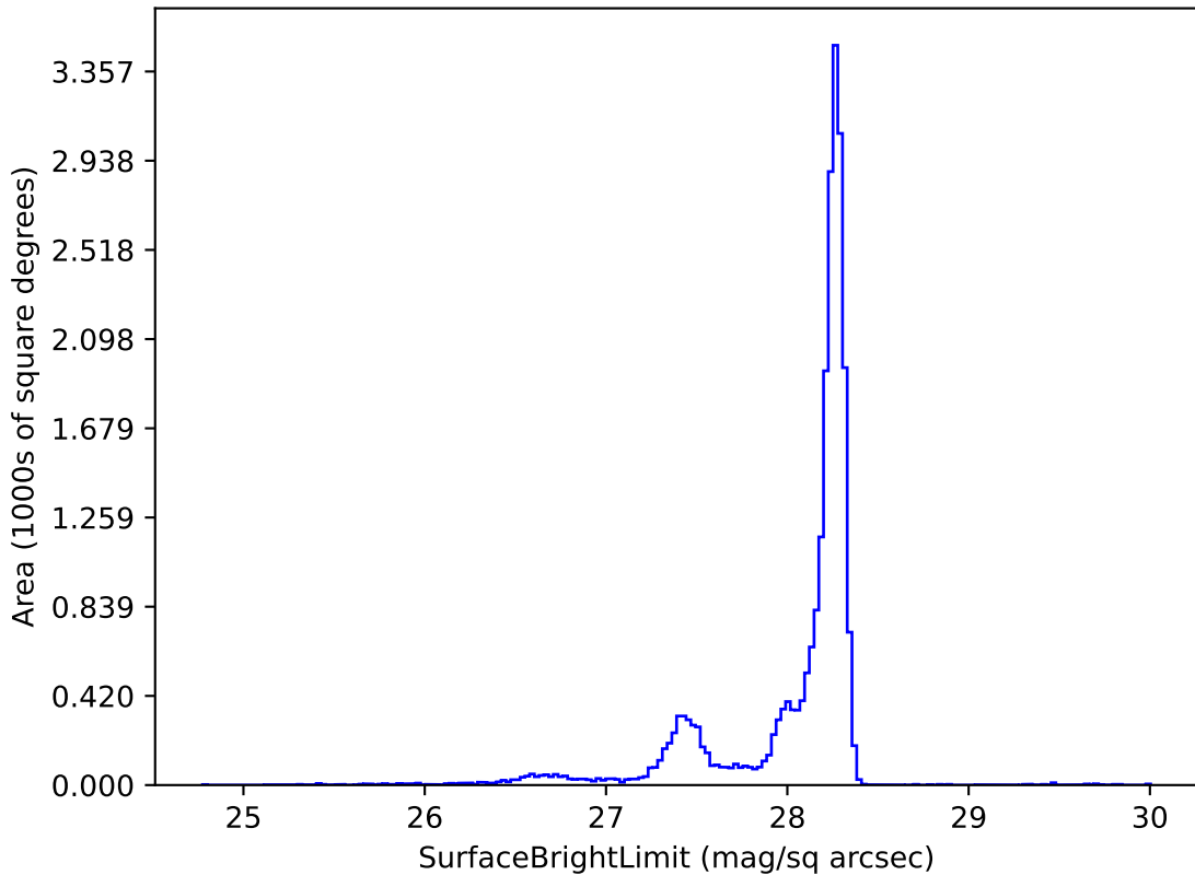
no_long_v3.4_10yrs y: SurfaceBrightLimit
