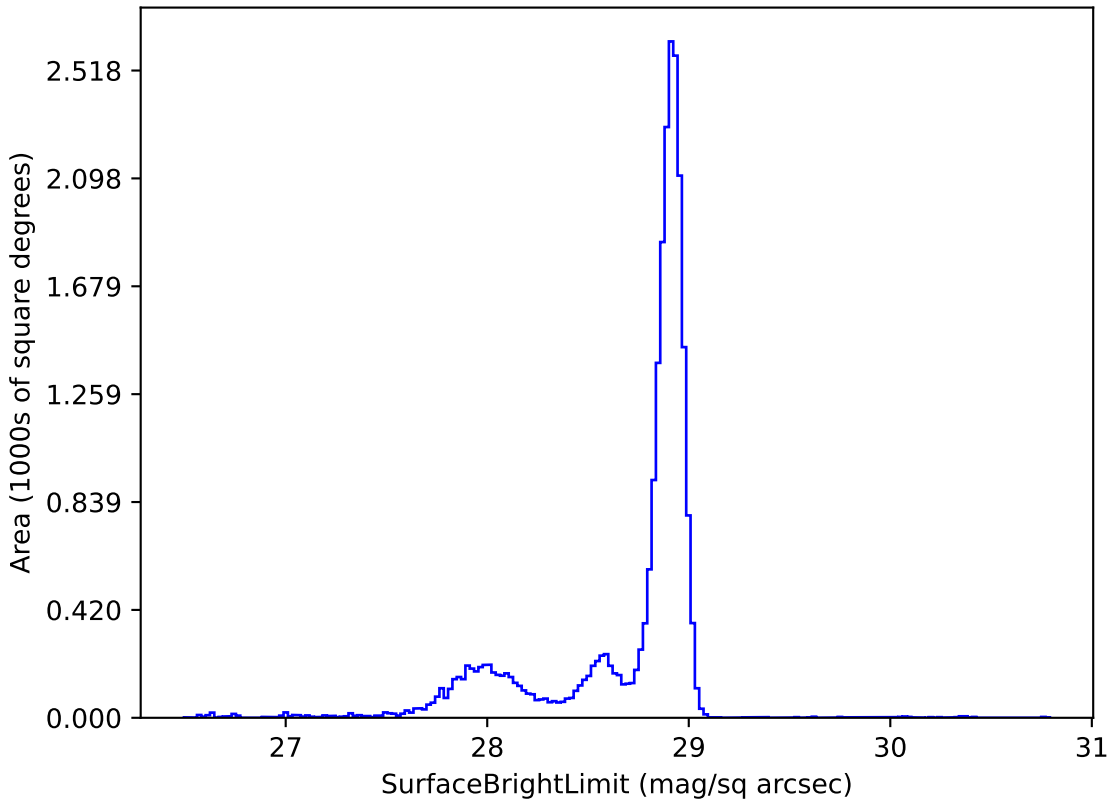
no_long_v3.4_10yrs u: SurfaceBrightLimit
