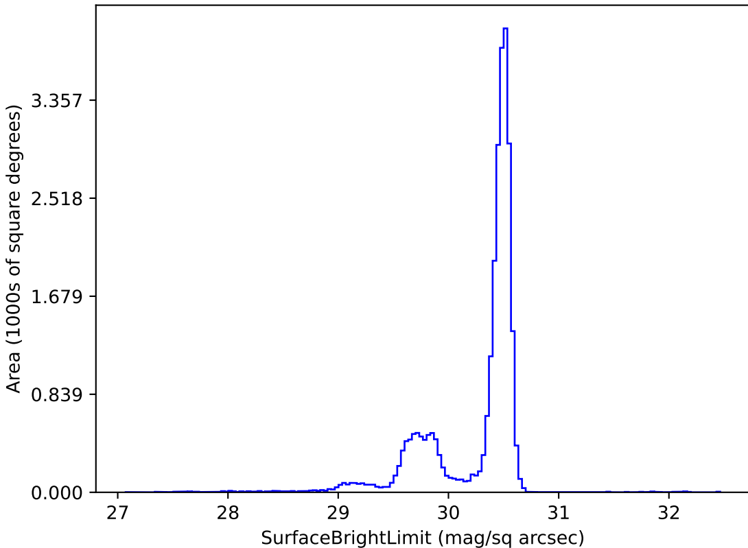
no_long_v3.4_10yrs r: SurfaceBrightLimit
