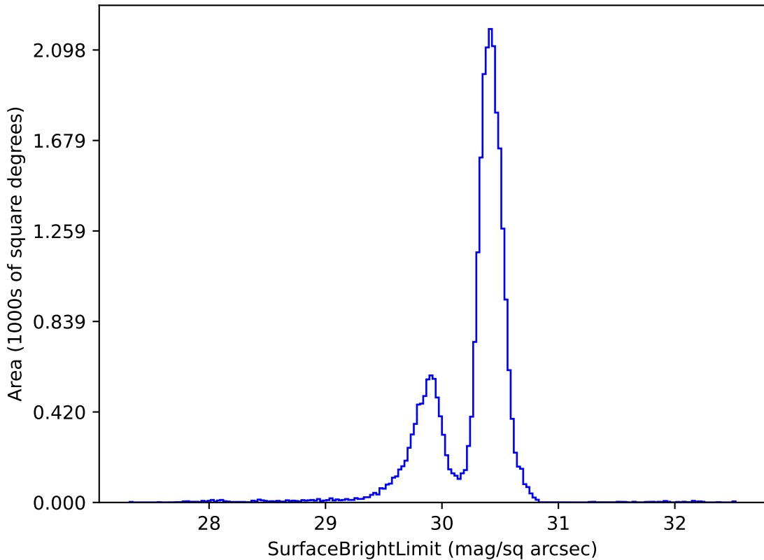
no_long_v3.4_10yrs g: SurfaceBrightLimit
