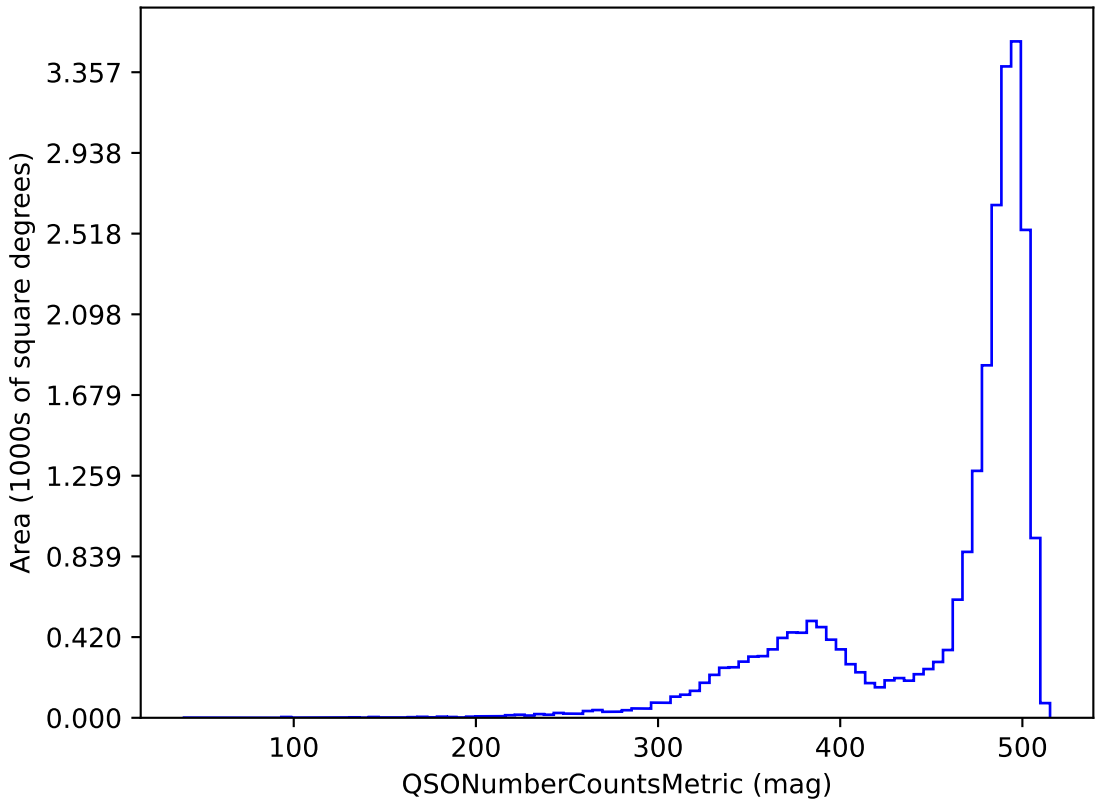
no_long_v3.4_10yrs z band and non-DD: QSONumberCountsMetric
