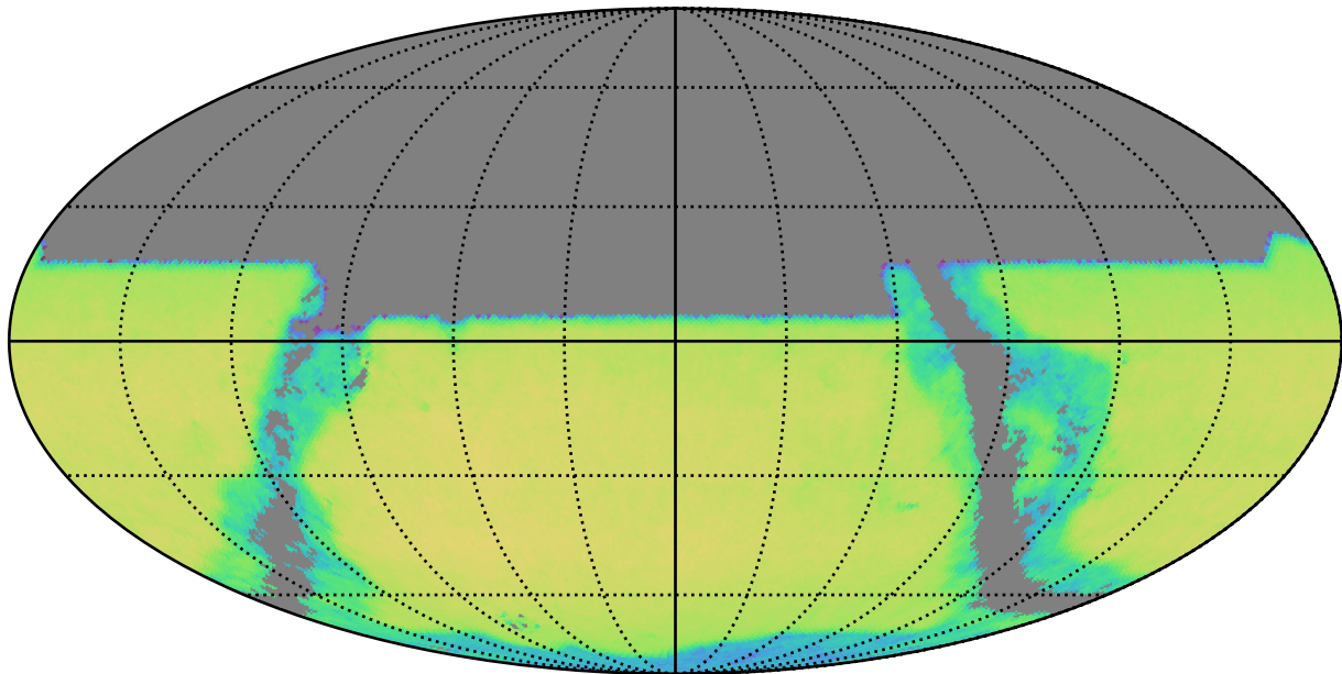
no_long_v3.4_10yrs y band and non-DD: QSONumberCountsMetric
