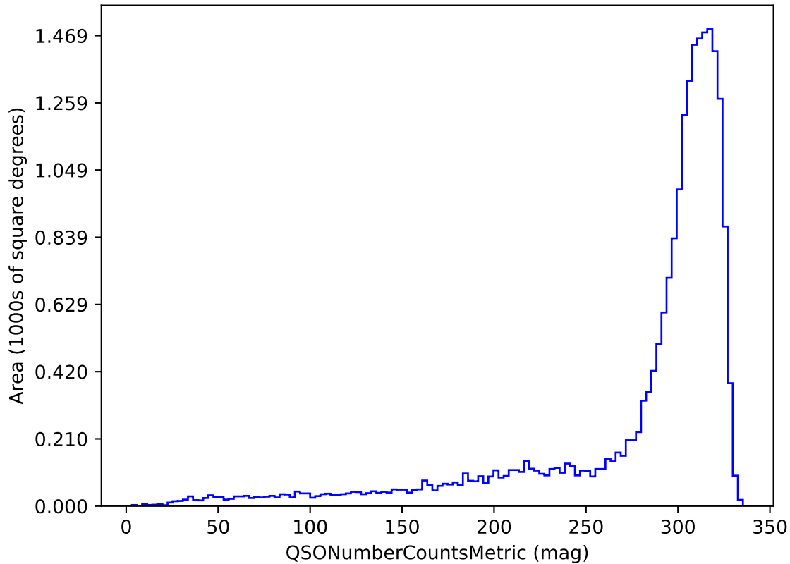
no_long_v3.4_10yrs u band and non-DD: QSONumberCountsMetric
