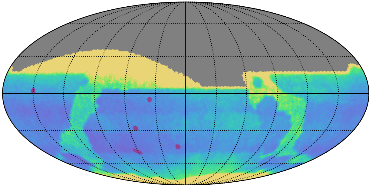
no_long_v3.4_10yrs : Proper Motion Uncert @ 24.0
