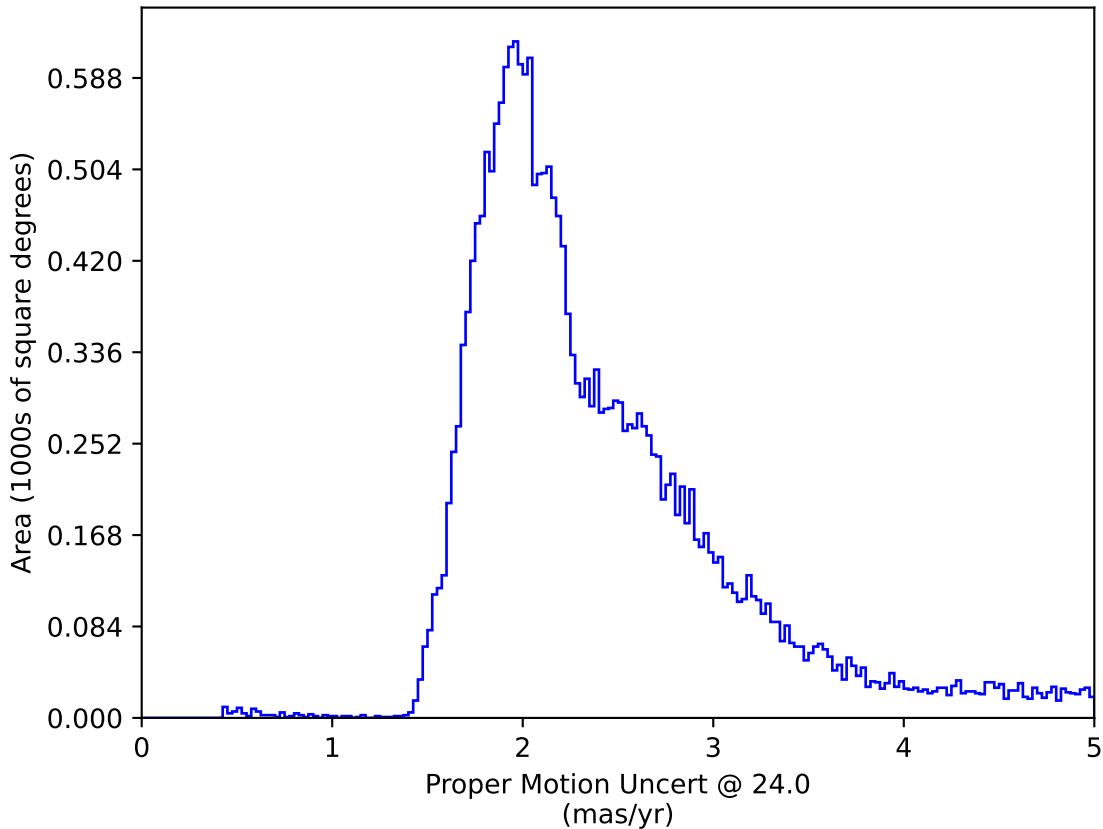
no_long_v3.4_10yrs : Proper Motion Uncert @ 24.0
