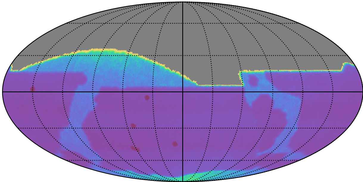
no_long_v3.4_10yrs : Proper Motion Uncert @ 20.5
