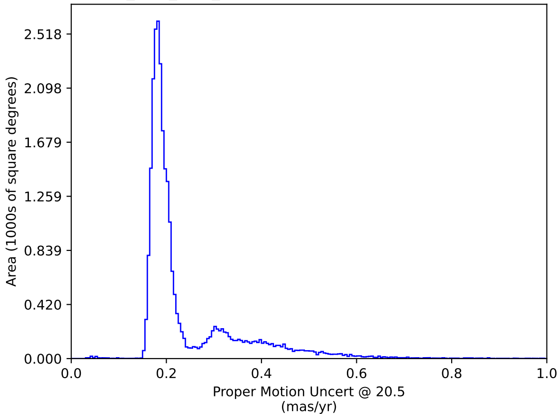
no_long_v3.4_10yrs : Proper Motion Uncert @ 20.5
