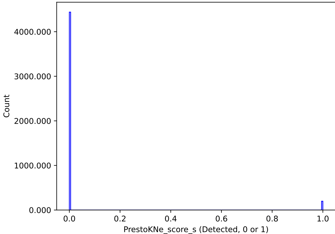
no_long_v3.4_10yrs : PrestoKNe_score_s
