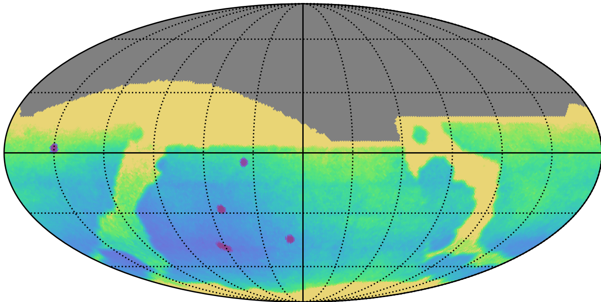
no_long_v3.4_10yrs : Parallax Uncert @ 24.0
