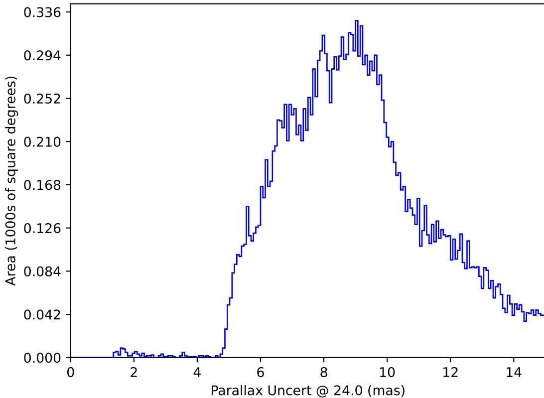
no_long_v3.4_10yrs : Parallax Uncert @ 24.0
