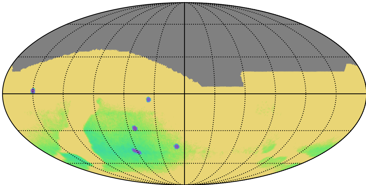
no_long_v3.4_10yrs : Parallax Uncert @ 22.4
