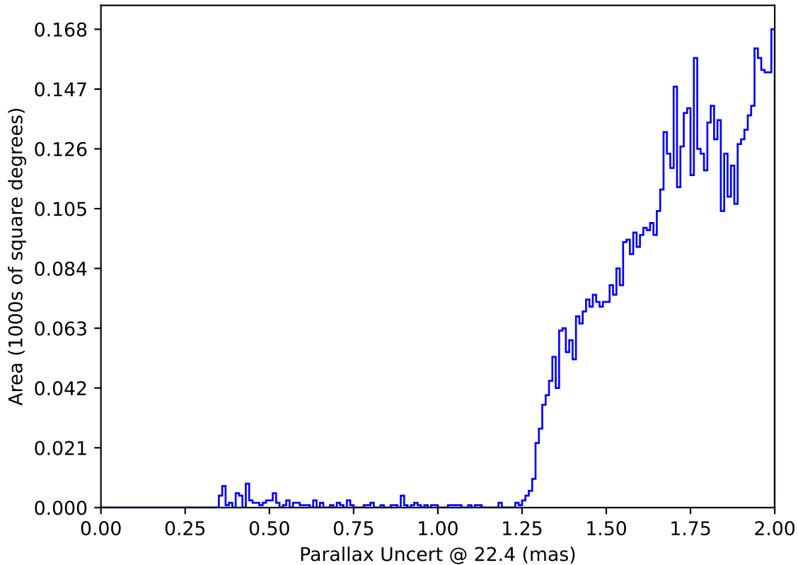
no_long_v3.4_10yrs : Parallax Uncert @ 22.4
