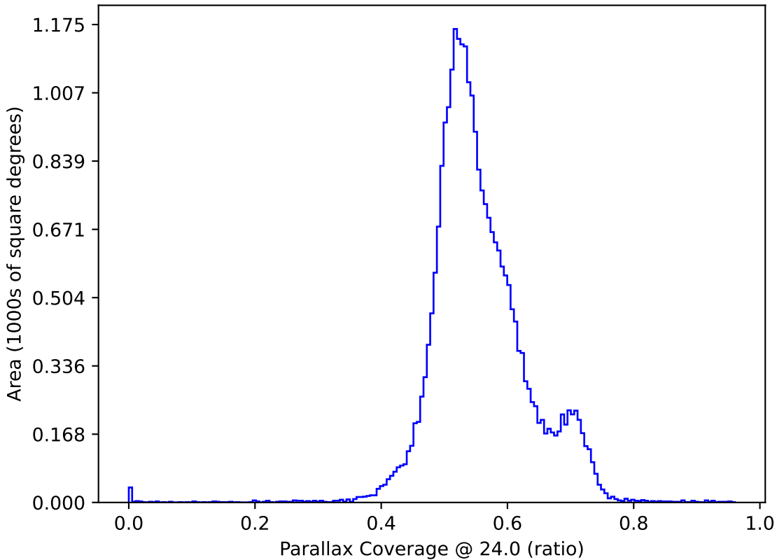
no_long_v3.4_10yrs : Parallax Coverage @ 24.0
