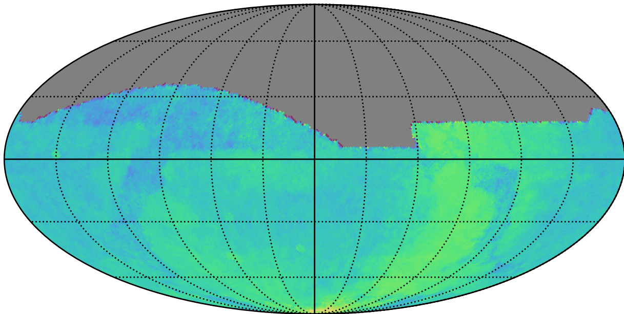
no_long_v3.4_10yrs : Parallax Coverage @ 22.4
