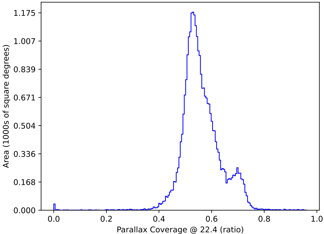
no_long_v3.4_10yrs : Parallax Coverage @ 22.4
