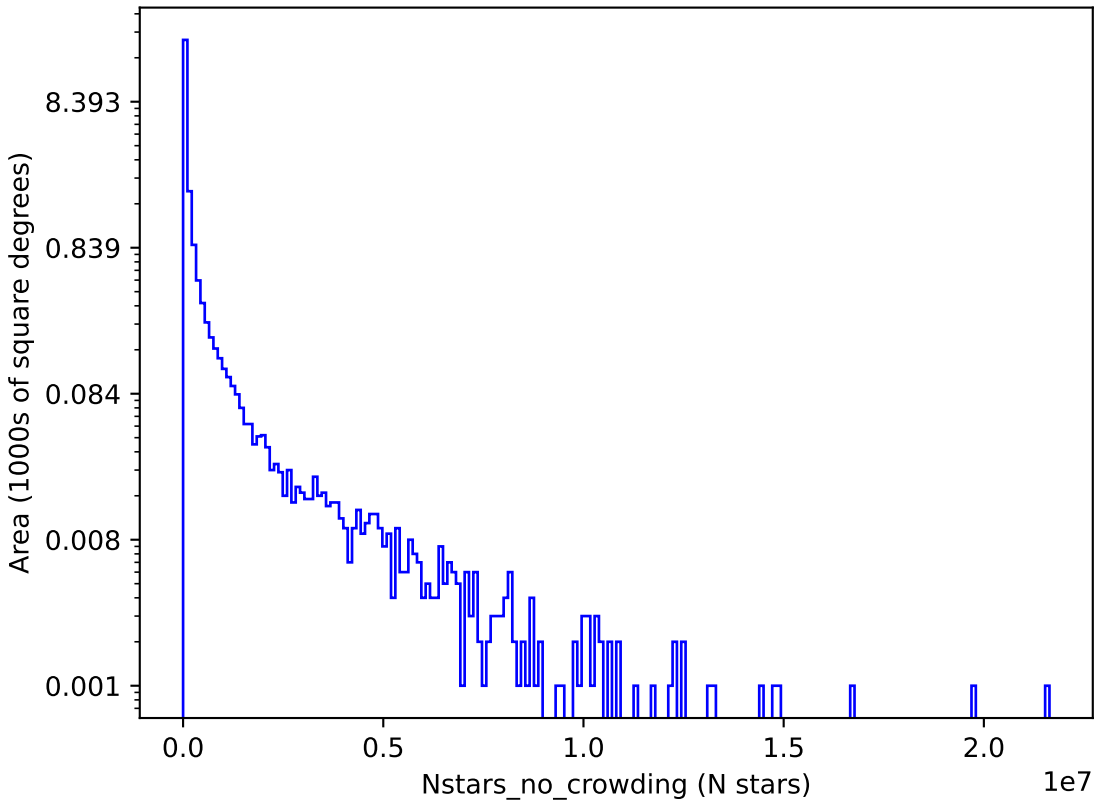
no_long_v3.4_10yrs r: Nstars_no_crowding
