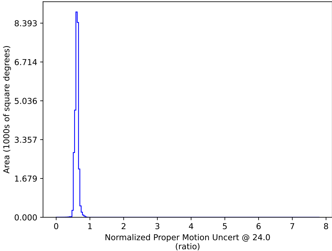
no_long_v3.4_10yrs : Normalized Proper Motion Uncert @ 24.0
