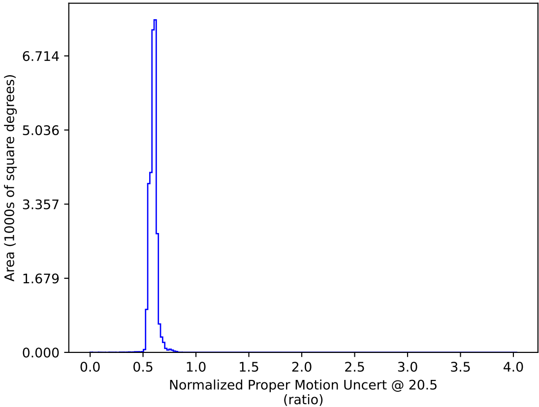
no_long_v3.4_10yrs : Normalized Proper Motion Uncert @ 20.5
