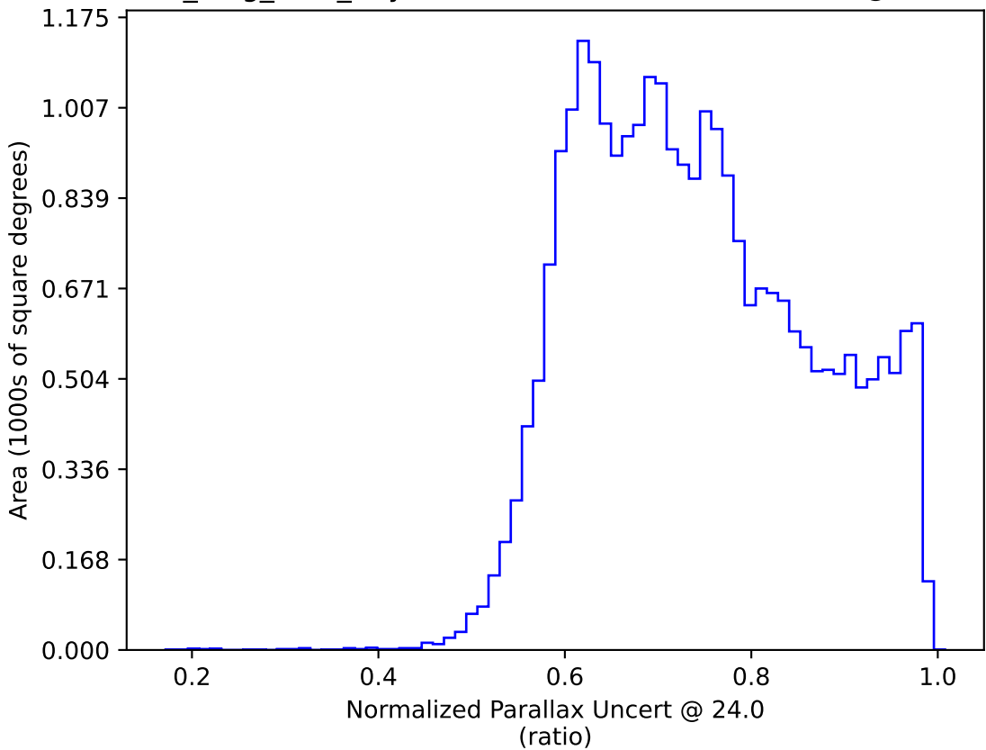
no_long_v3.4_10yrs : Normalized Parallax Uncert @ 24.0
