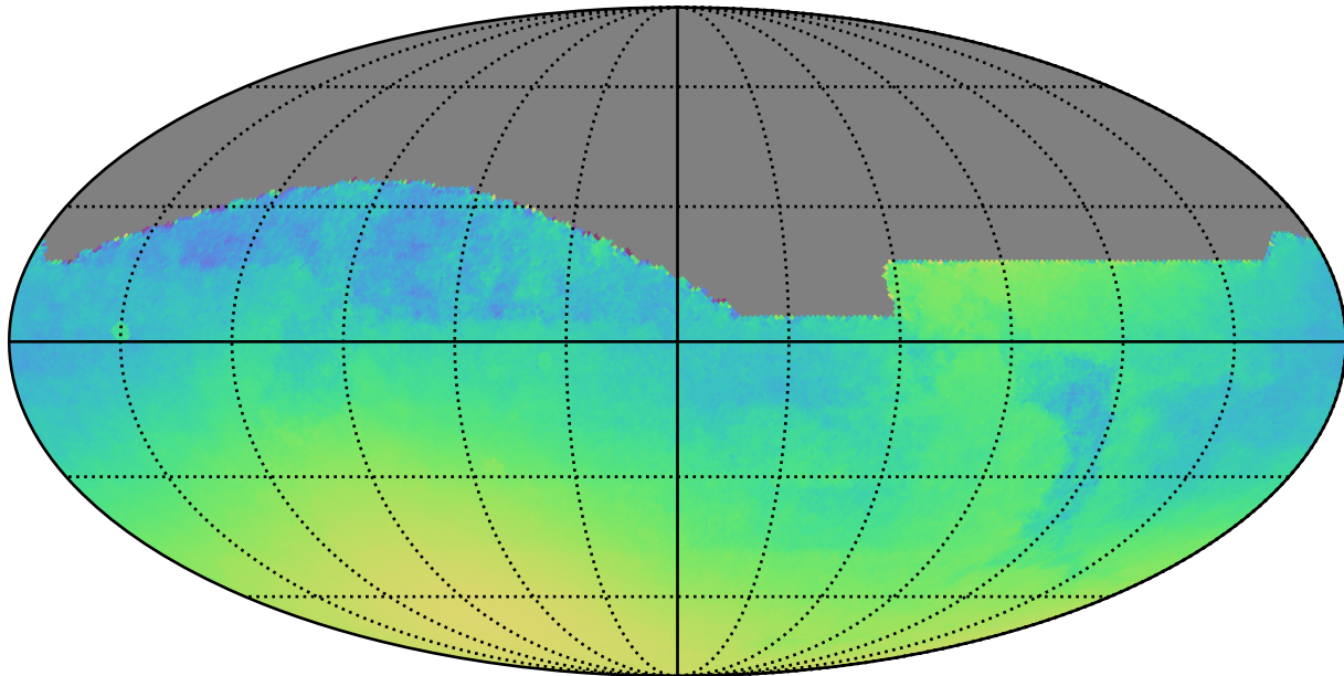
no_long_v3.4_10yrs : Normalized Parallax Uncert @ 22.4
