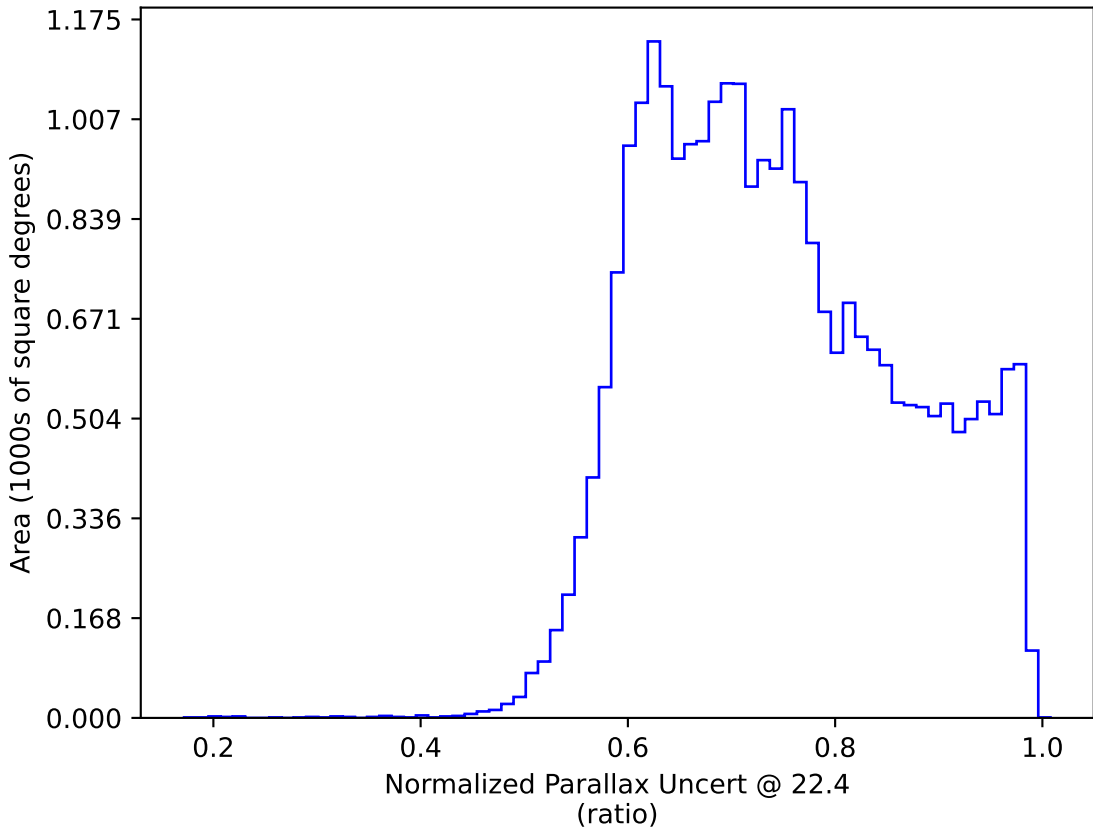
no_long_v3.4_10yrs : Normalized Parallax Uncert @ 22.4
